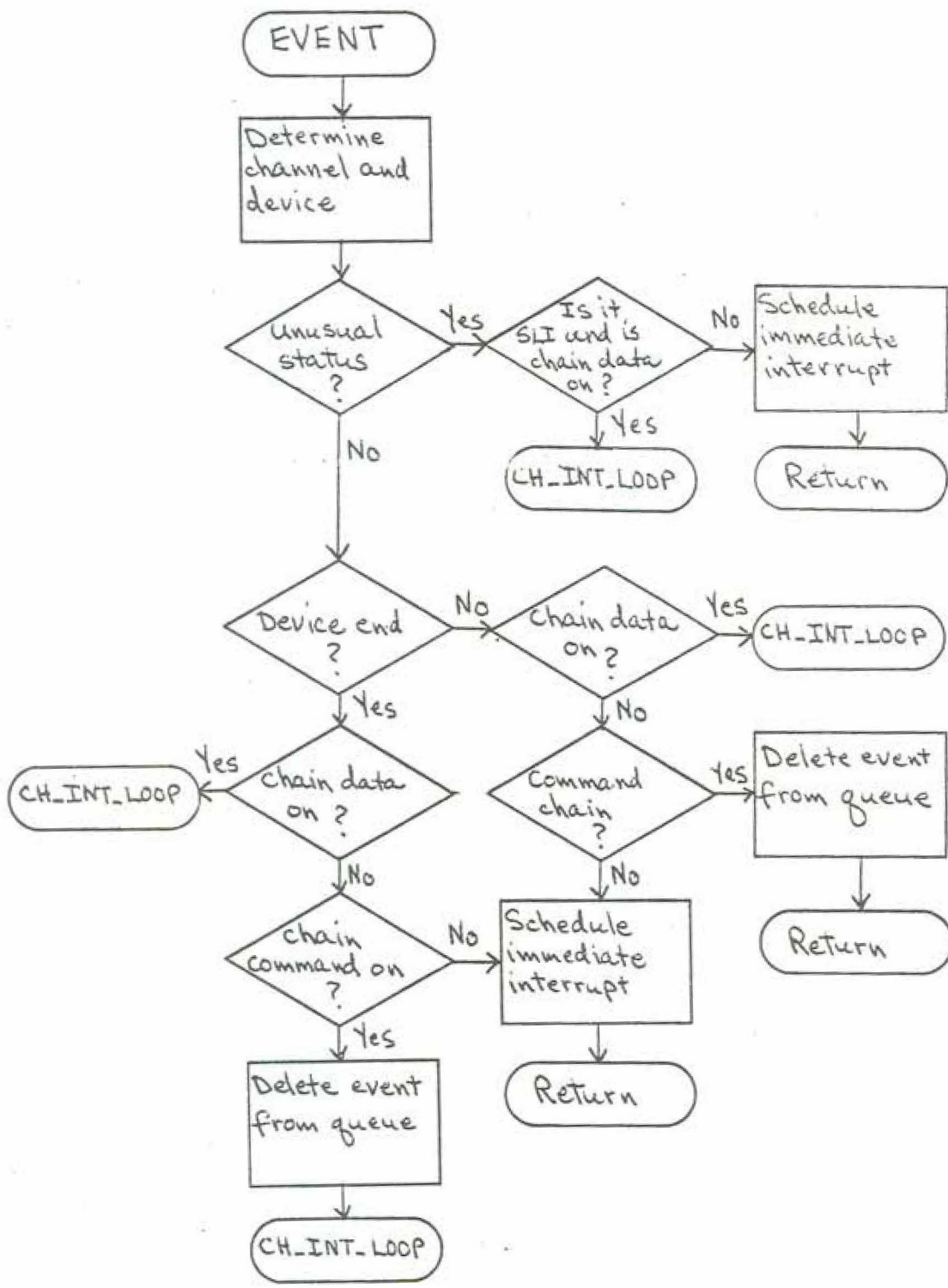
Figure C-11 : Event Processing
