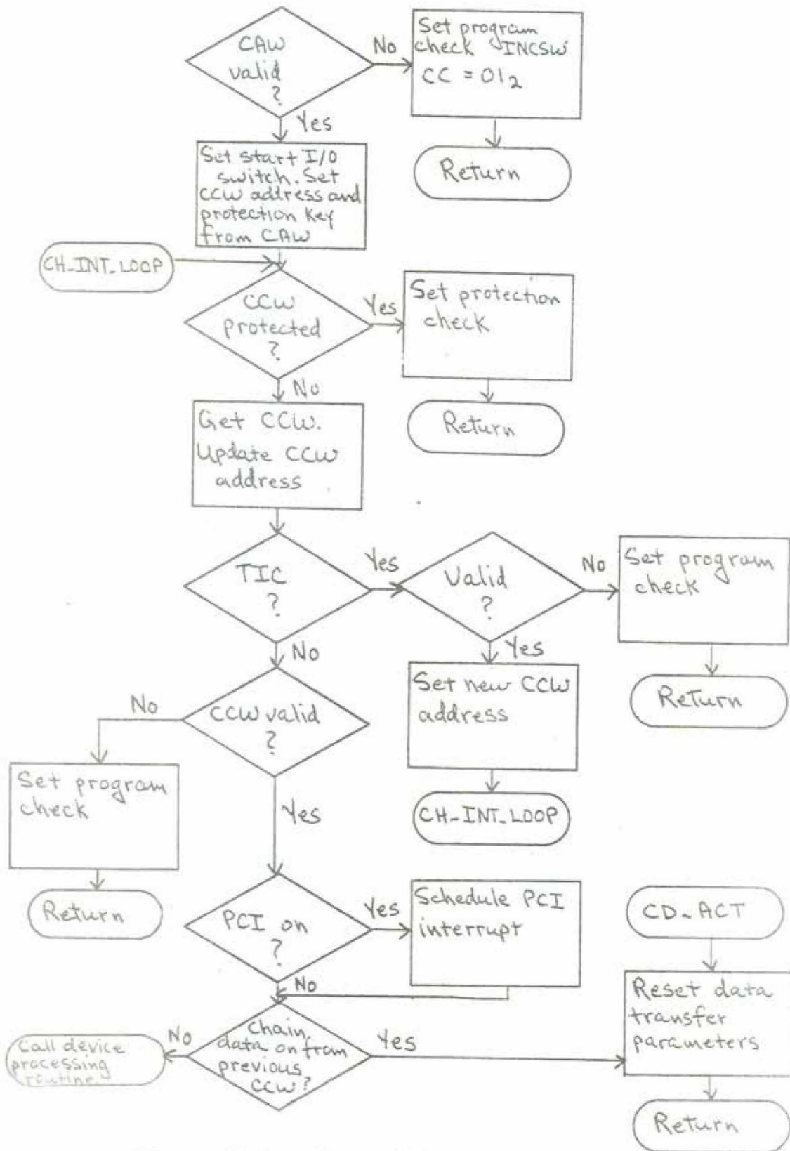
Figure C-9 : Channel Interpreter
