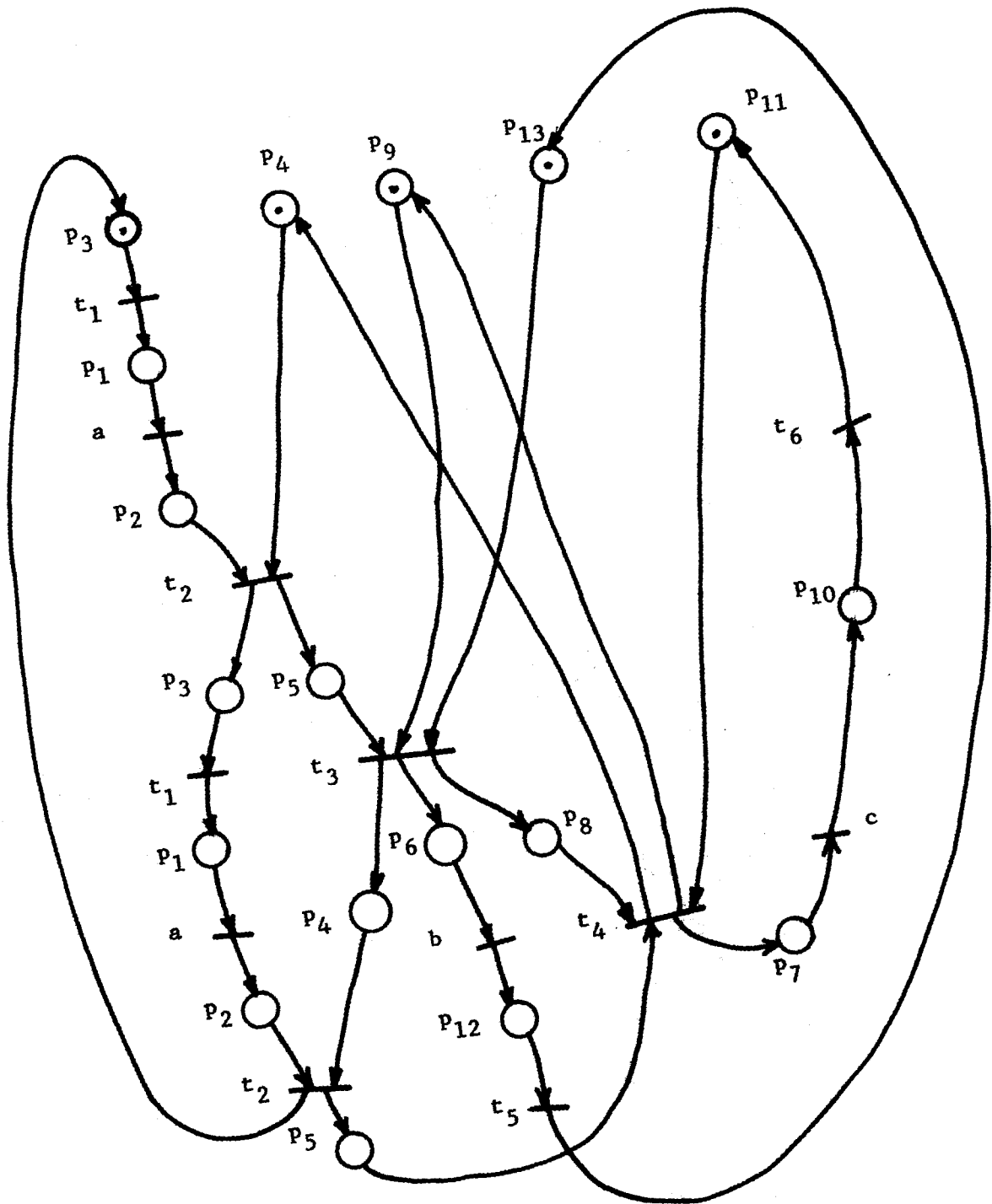
Figure 6.1.10(b) Steady State Equivalent Net
