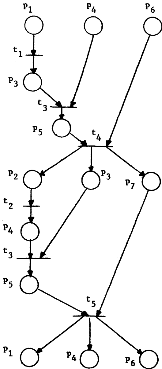
Cyclic Frustrum of \mathcal{B} .
