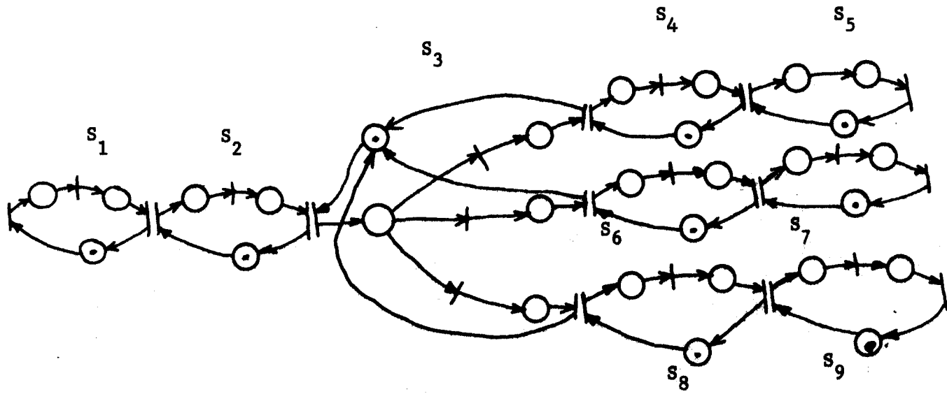
Figure 3.1.6 State Machine components of net in Figure 3.1.5
