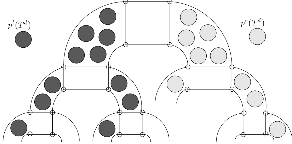
Figure 3-4: Paths used by p_i^l(T^d) and p_i^r(T^d) .
