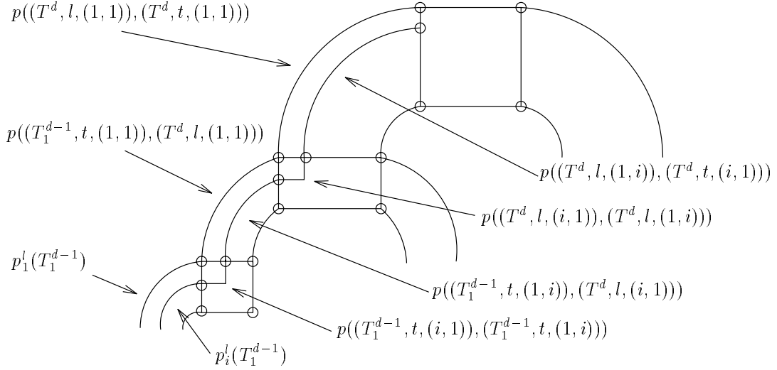
Figure 3-5: Construction of p_i^l(T^d) .
