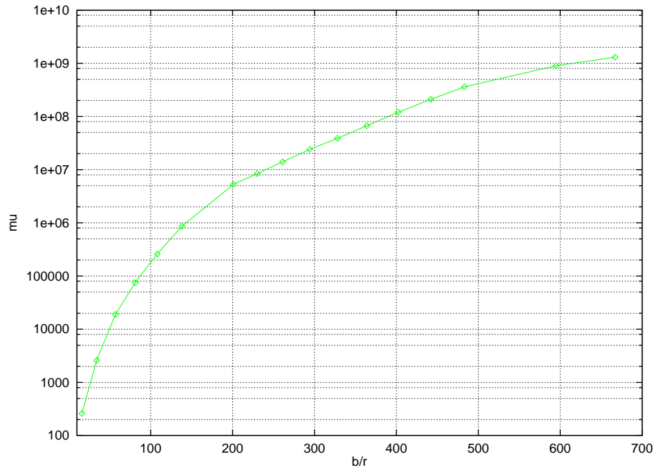
Figure 5-3: \mu as a function of b/r , the number of circuits a link can simultaneously carry.
