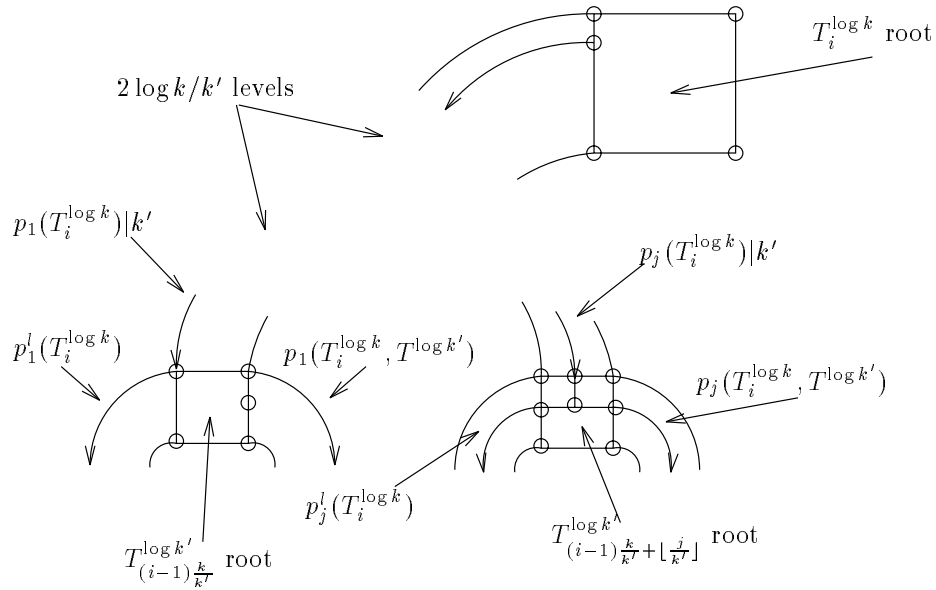
Figure 3-6: Construction of p(T_i^{\log k}, T^{\log k'}) .
