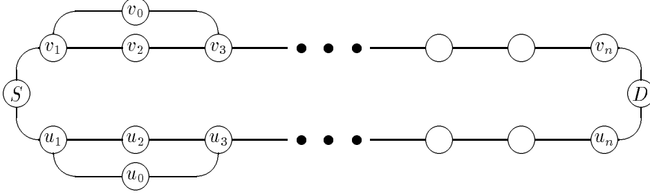
Figure 3-9: Network G with capacity 1 on each link.
