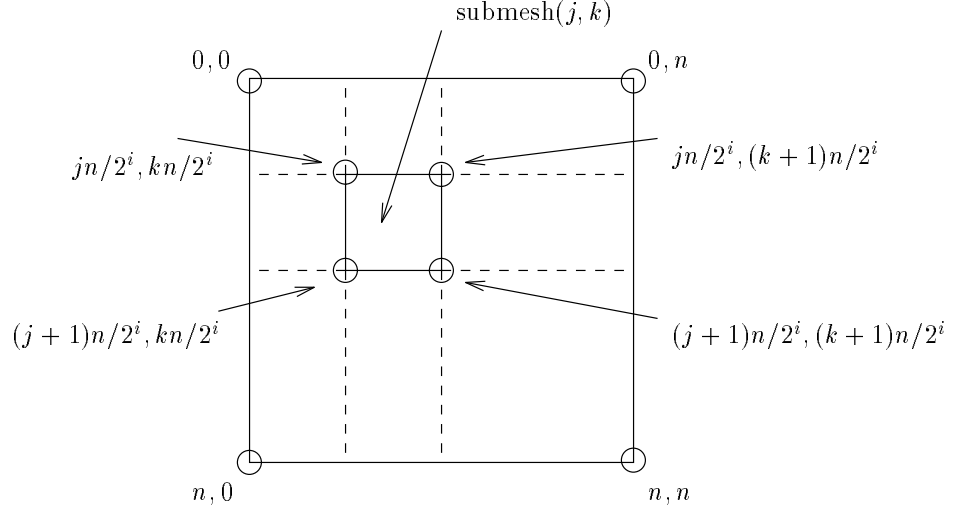
Figure 3-2: Submesh j, k , for 0 \leq j < 2^i and 0 \leq k < 2^i , from the division of (n + 1) \times (n + 1) mesh into 4^i submeshes of size (\frac{n}{2^i} + 1) \times (\frac{n}{2^i} + 1) .
