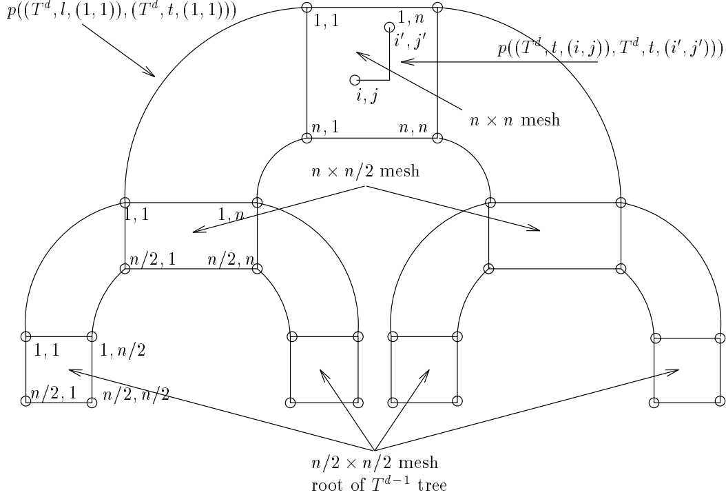
Figure 3-3: Structure and notation for n \times n tree of meshes.
