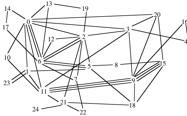
Figure 6-1: Topology of an existing commercial network.
