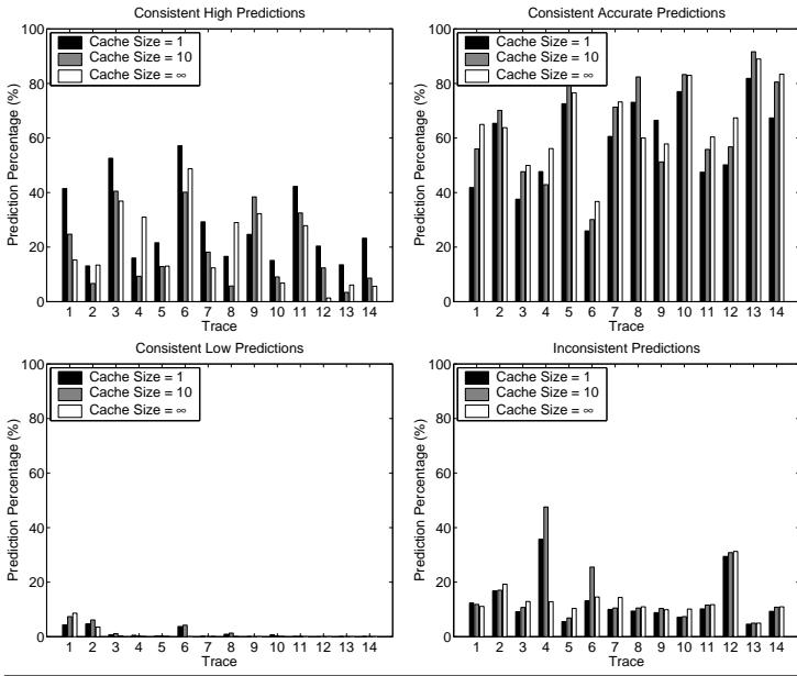
Figure 14 Concrete Trace Representation — Consistent High/Accurate/Low and Inconsistent Prediction Percentages.
