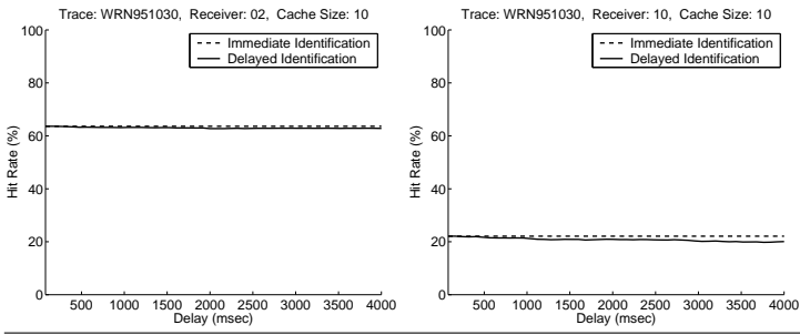
Figure 9 Virtual Link Trace Representation — Prediction hit rates wrt loss identification delay, cache of size 10 (Trace WRN951030).
