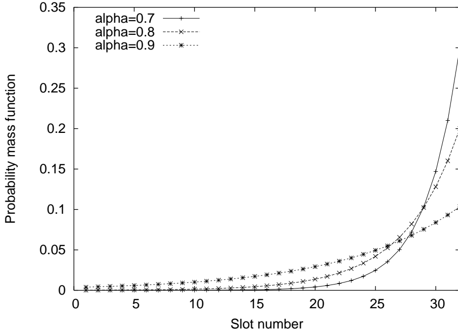
Figure 1: The probability distribution for the contention slot number that each Sift station chooses. We show various values of \alpha , the parameter of the distribution.
