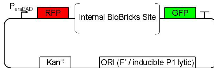
Figure 4: PoPS screening plasmid schematic.
