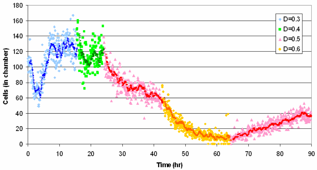
Figure 11: Cell counts in the sorting chamber for a 90hr sortostat run with device operating in normal chemostat mode, samples were captured at 3 minute intervals. The dilution rate was varied from 0.3\text{hr}^{-1} to 0.6\text{hr}^{-1} and culture density responded appropriately. The darker lines are a moving average with a ten time point window.
