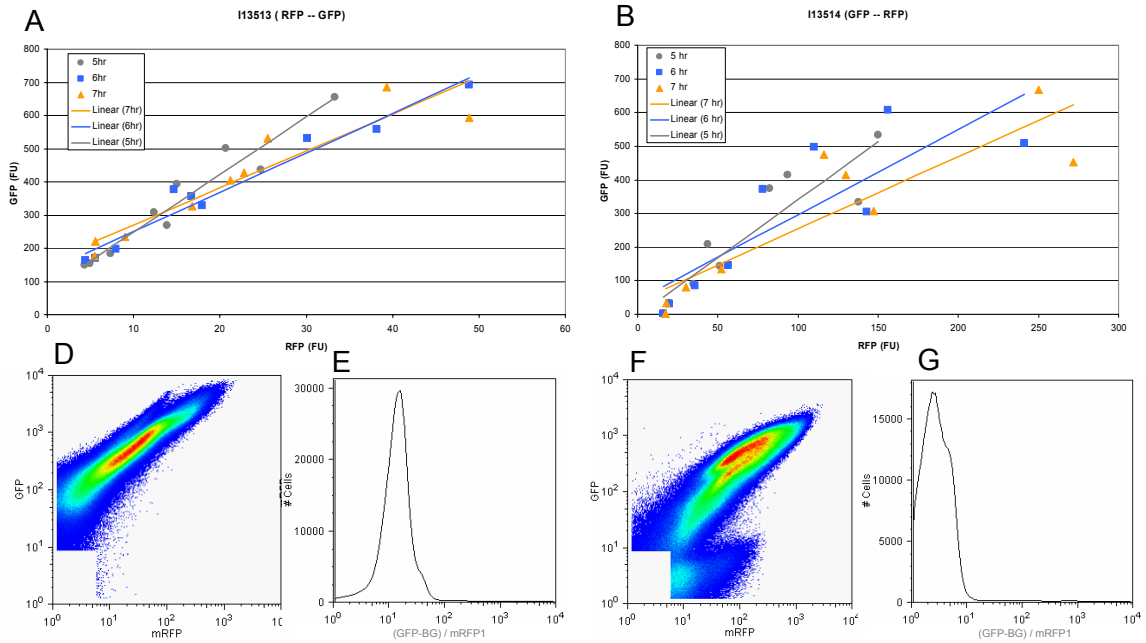
Figure 8: Figure 8 (A & B) shows the geometric mean of the GFP and mRFP1 fluorescence intensities in relative fluorescence units across three time points and six arabinose concentrations. The lines shown are the linear best fit for each time point. The dot plots for BBa_I13513(D) and BBa_I13514(F) display the complete (all arabinose concentrations and times) single cell data set concatenated on a single plot. The histograms show the ratio of GFP/RFP corrected for background GFP for BBa_I13513 (E) and BBa_I13514 (G) for the complete data set.
