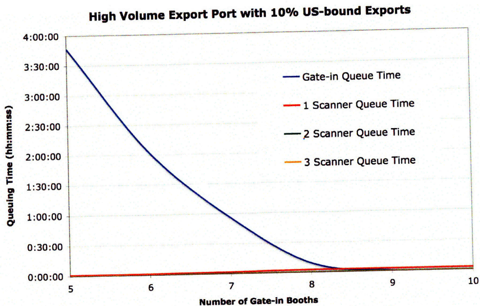
Figure 24. Queue Times for High Volume Export Port with 10% US-bound Exports
