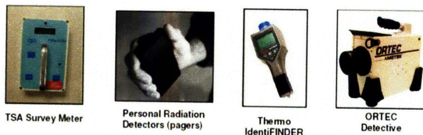
Figure 6. Sample Hand-held Equipment for SFI Ports
