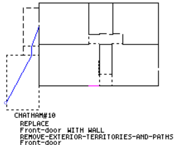
Figure 8.17: Starting design with side door as perceived main entry. Path is from usual approach (○) to side door.
