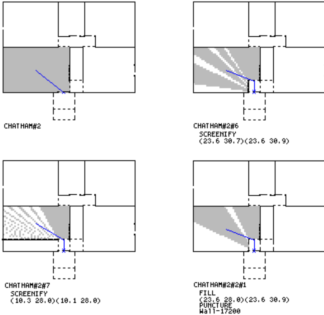
Figure 8.16: Starting design (#2), solutions for Living visual openness and path from front door: 0.3 < \text{visual openness} < 0.8 , and 10 \text{ degrees} < \text{path direction change} < 120 \text{ degrees} . Shaded areas are visible; * is viewpoint; path is from front door to center of Living.
